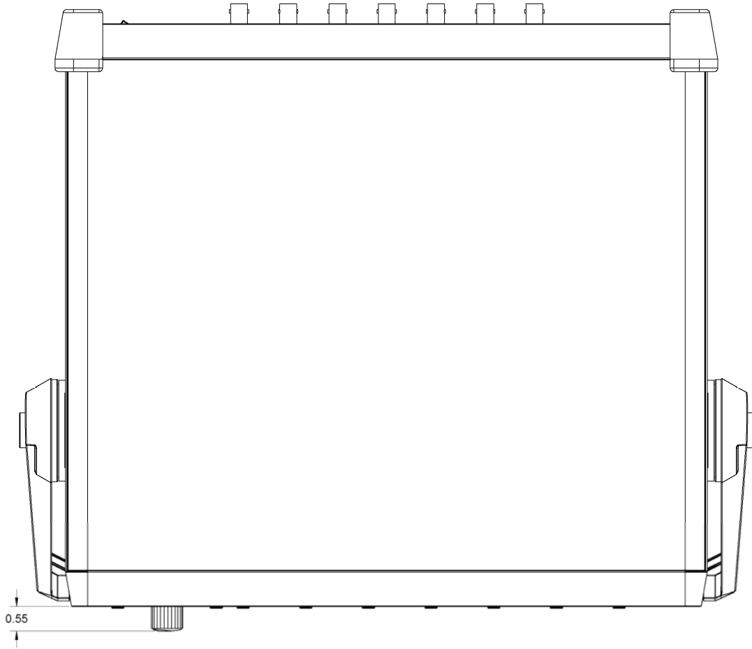
Figure 20 3/4 Rack Top View With Display
