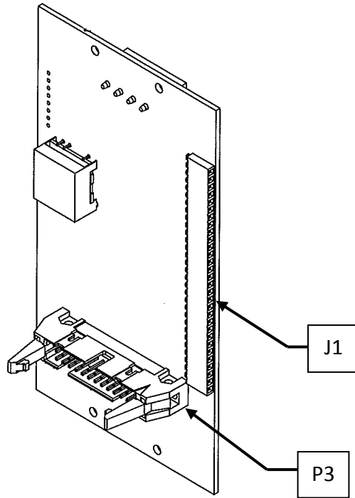
Figure 6 Display Module Back Plane PCB, Front View
