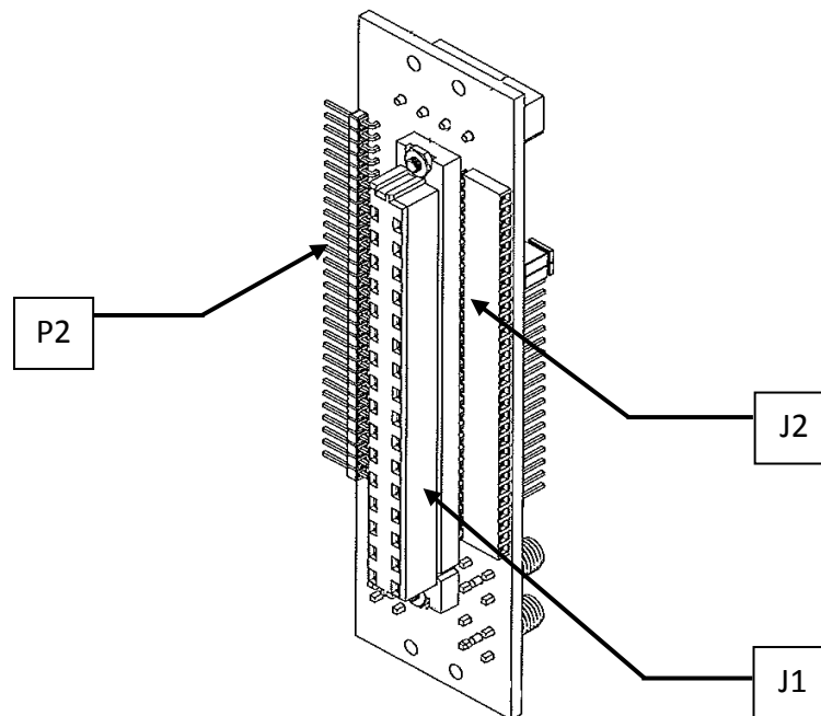
Figure 2 Measuring Channel Back Plane PCB, Front View
